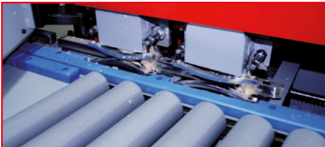
Polieraggregat buffing unit
